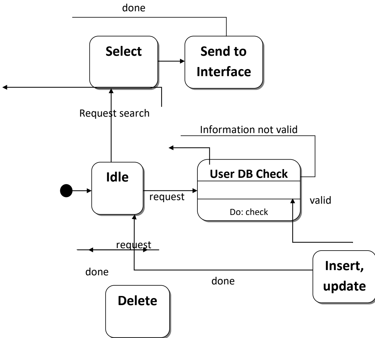
Fig: State diagram (Database Class)
