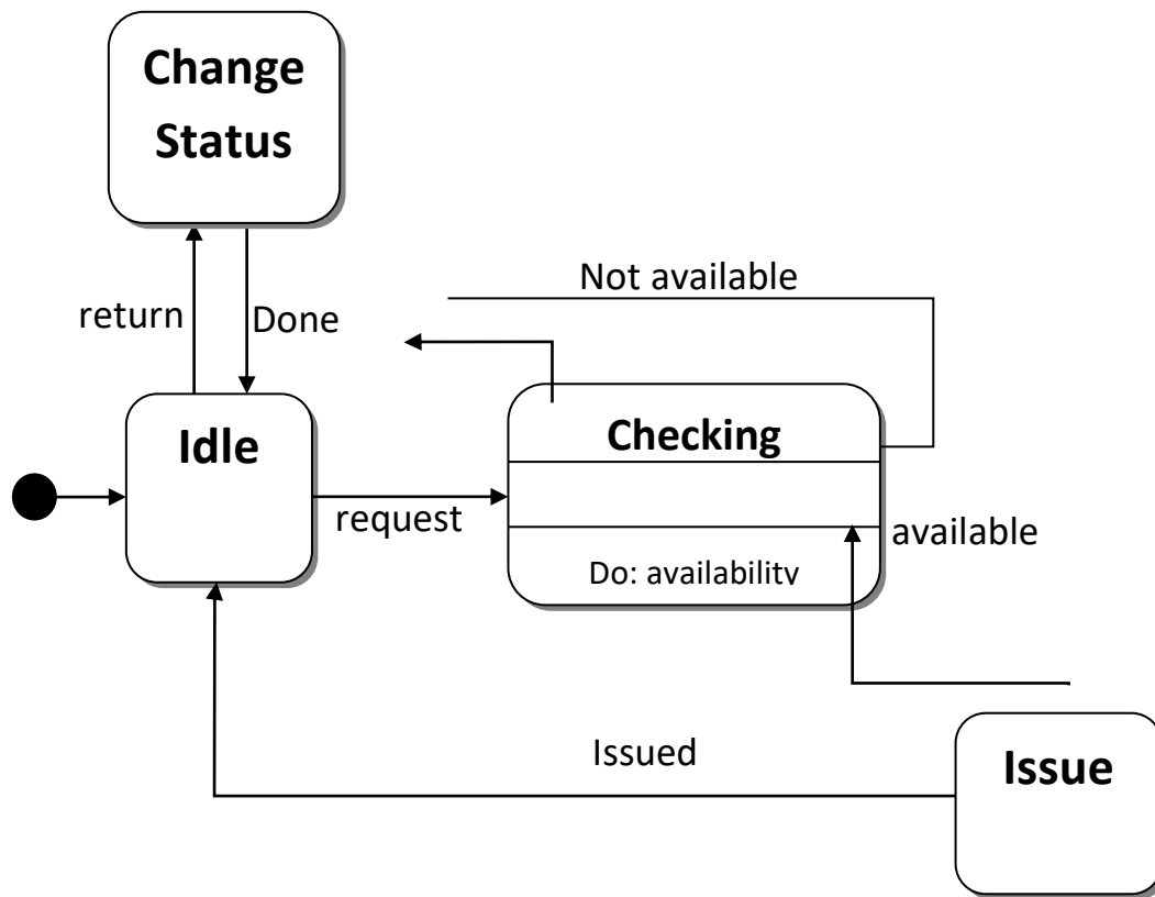
Fig: State diagram (Item Class)
