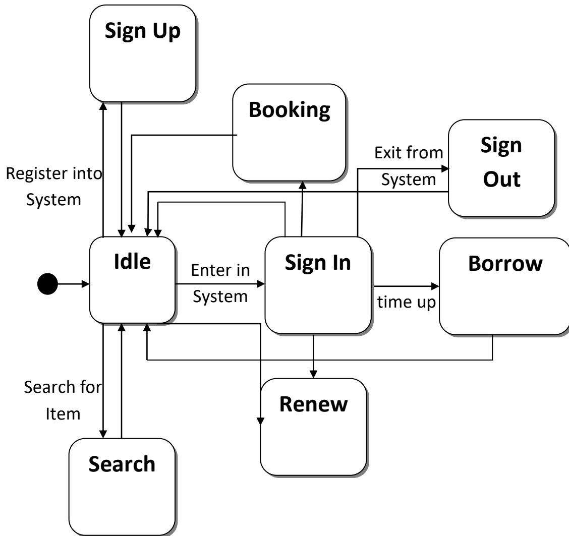
Fig: State diagram (User Class)
